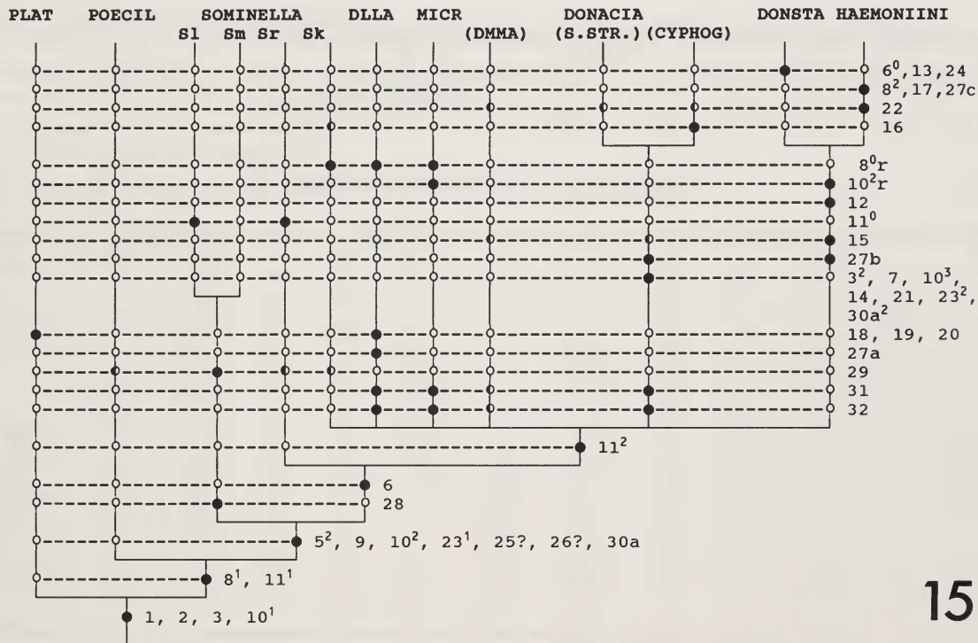
FIGURE 15. Reconstructed phylogeny of genera and some taxa of Donaciinae not assigned to genus. PLAT = Plateumaris ; POECIL = Poecilocera ; S1 = Sominella longicornis ; Sm = Sominella macrocnemia ; Sr = Sominella reticulata ; Sk = Sominella kraatzi ; DLLA = Donaciella ; MICR = " Donacia " microcephala ; DMMA = D. (Donaciomima) ; CYPHOG = Donacia (Cyphogaster) ; DONSTA = Donaciasta . ● = apomorphic character states; ○ = plesiomorphic character states; half-circles = specimens (or taxa) with both states occurring in that taxon; r = reversal.
